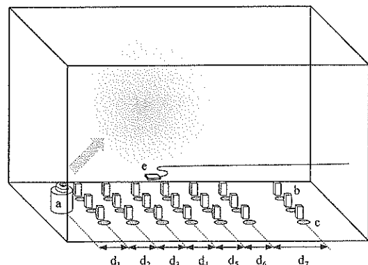
Fig.2. Locations of the fogger, cuvettes containing APF solution, and E. coli -attached membrane filters in the fogging experiment room (107m 3 ). a, fogger; b, cuvette; c, membrane filters; d 1 -d 6 , 0.5m; d 7 , 2.5m; e, hygro-thermometer.
