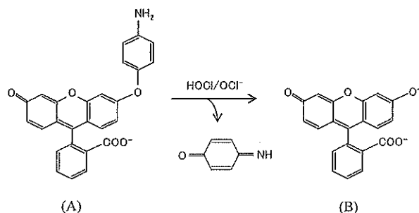
Fig.1. Scheme of conversion of APF (A) to strongly fluorescent fluorescein (B) by HOCl/OCl - .
